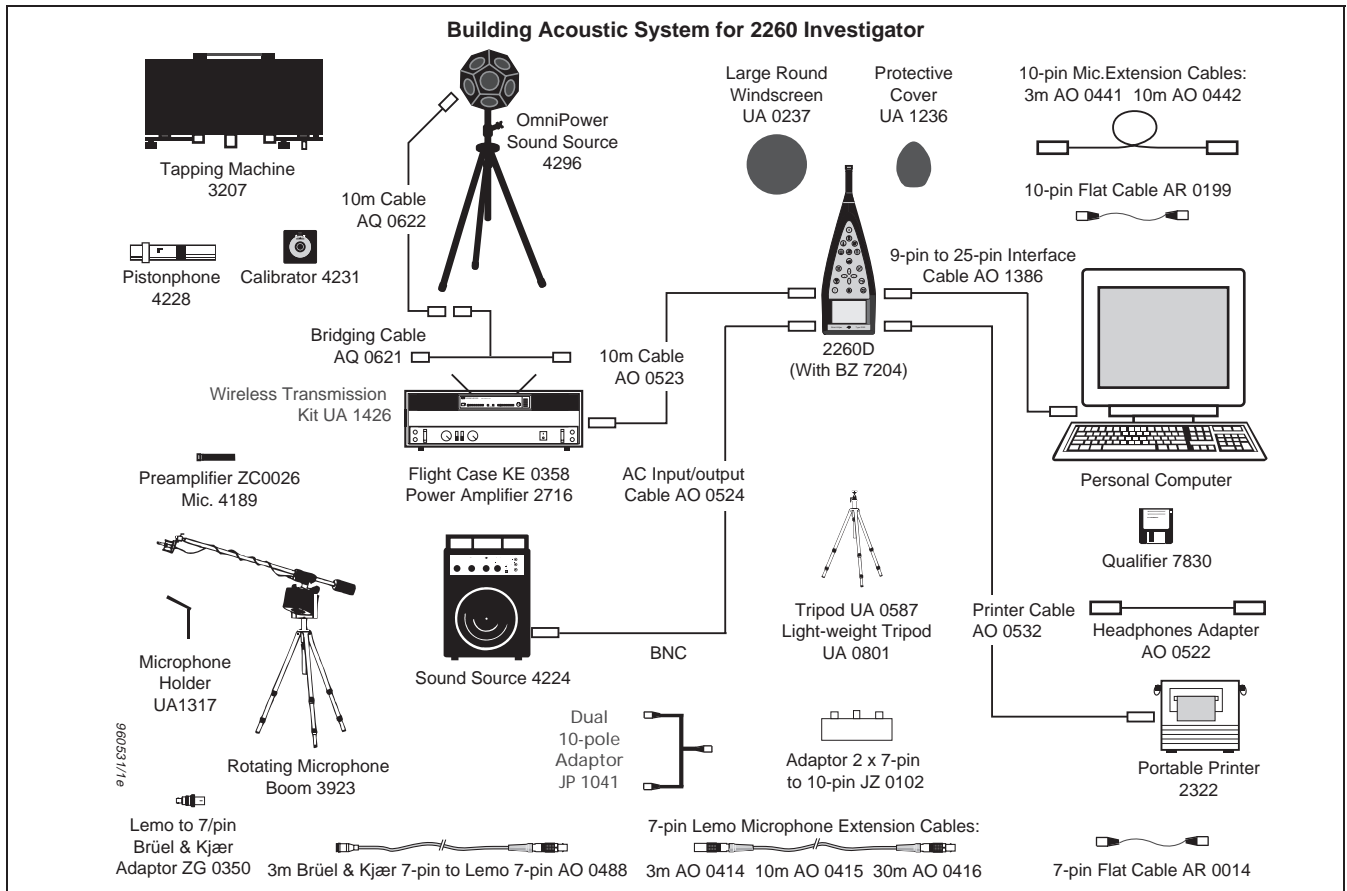
Fig. 14 Accessories for Investigator Types 2260D and 2260G
