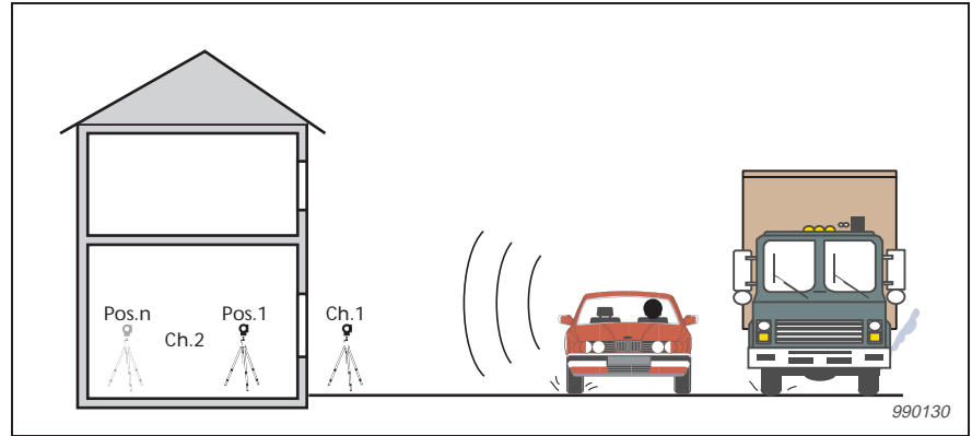
Fig. 11 Measuring sound pressure outside and inside the façade simultaneously – 2-channel measurement
