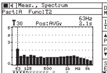
Fig. 3 Screen shot showing the spectrum of reverberation times
