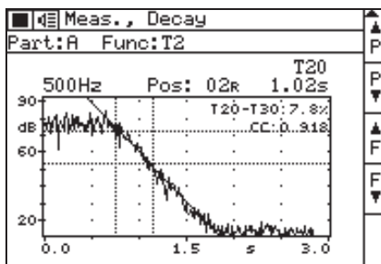
Fig. 4 Decay at 500Hz for a typical measurement
