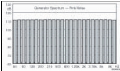
Fig. 5 1/3-octave spectrum of the internal generator output for pink noise set to 50 Hz – 10 kHz. Measured in 1/3-octaves 50 Hz – 10 kHz
