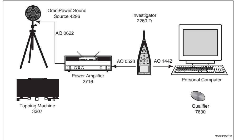
Fig. 1 Typical measurement setup also showing optional equipment available from Brüel & Kjær to cover your requirements for measuring and analysing architectural and building acoustics
